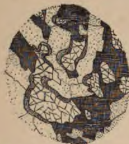
FIG. 15.—A new mineral (hornblende) forming as an intermediate "reaction rim" between the mineral having irregular fractures (olivine) and the dusty white mineral (lime-soda feldspar).
